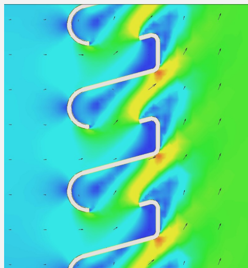
EFD simulation
